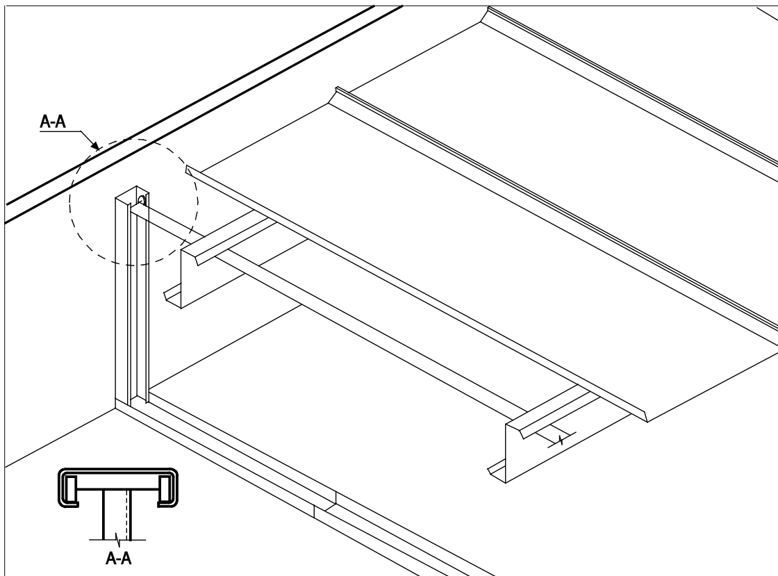
Figure 2 - Example of Lateral Restraint Test Device
